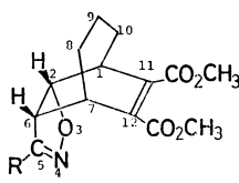
11 , R = C 6 H 5 , C 6 D 5 13 , R = C 6 H 5
